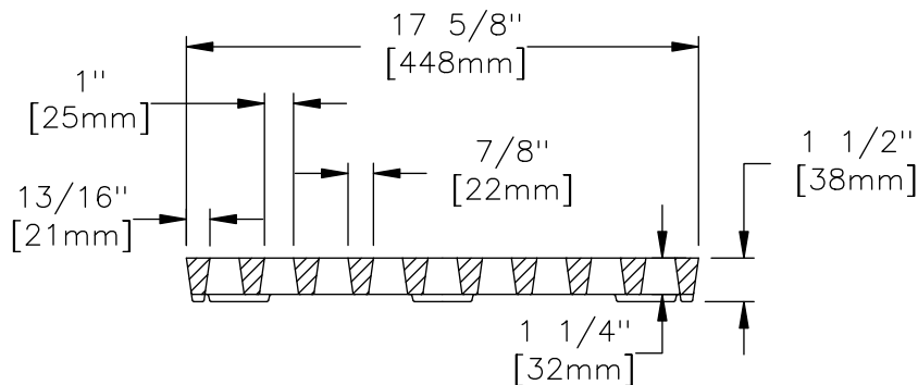
SECTION VIEW
