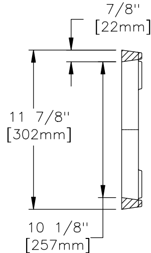
SECTION VIEW
